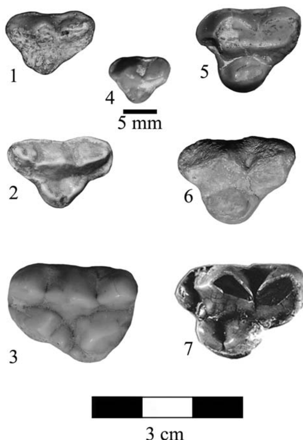
Fig. 2.—Comparison between the P4 of the Ailuropodinae with those of Ursavus and Indarctos species. 1: Agriarctos beatrix nov. sp. (Nombrevilla 2). 2: Agriarctos depereti Soblay (Soblay, cast T.F 167 Naturhistorisches Museum Basel). 3: Ailuropoda melanoleuca (MNCN-12831). 4: Ursavus brevirohinus (Can Llobateres, Crusafont & Kurtén 1976). 5: Indarctos vireti (Can Llobateres, Crusafont & Kurtén, 1976). 6: Indarctos arctoides (Batallones 3, MNCN-BAT-3'08.357. 7: Indarctos atticus (Crevillente 2, Montoya et al., 2001).
